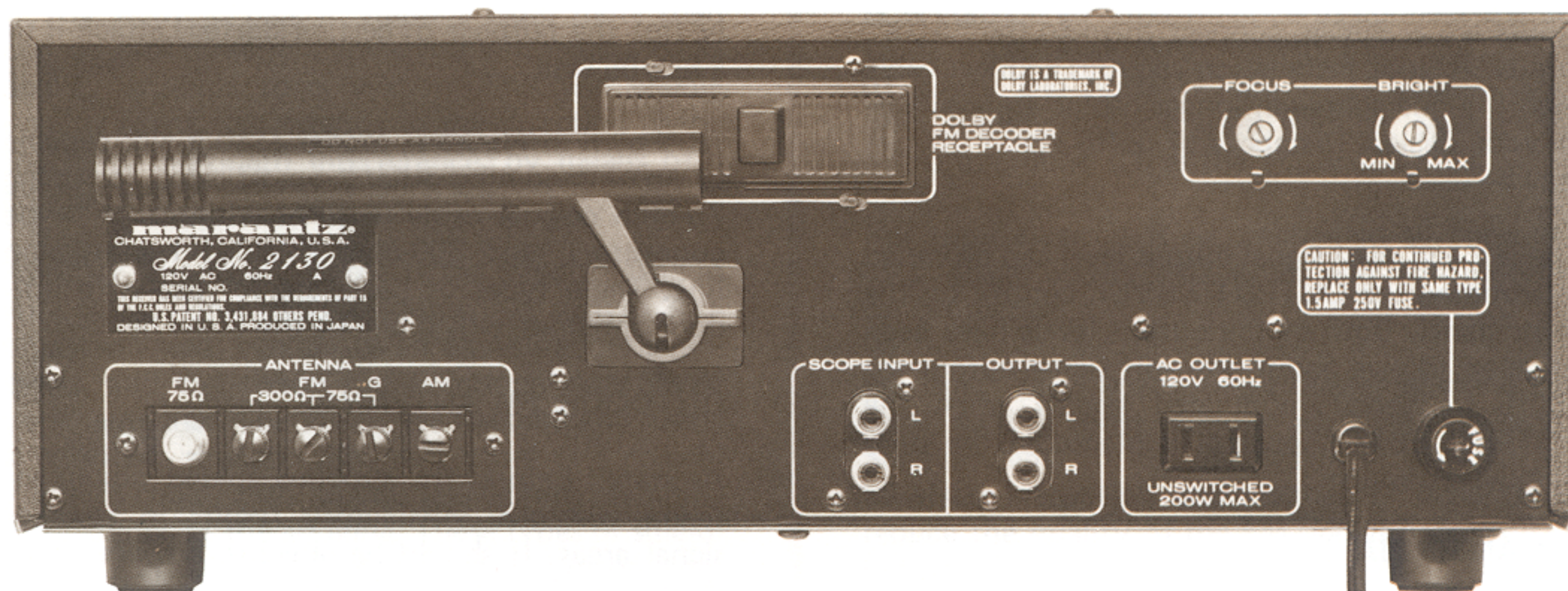
Figure 2. Rear Panel
