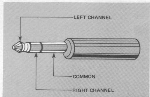
Figure 6 Stereophonic Plug
