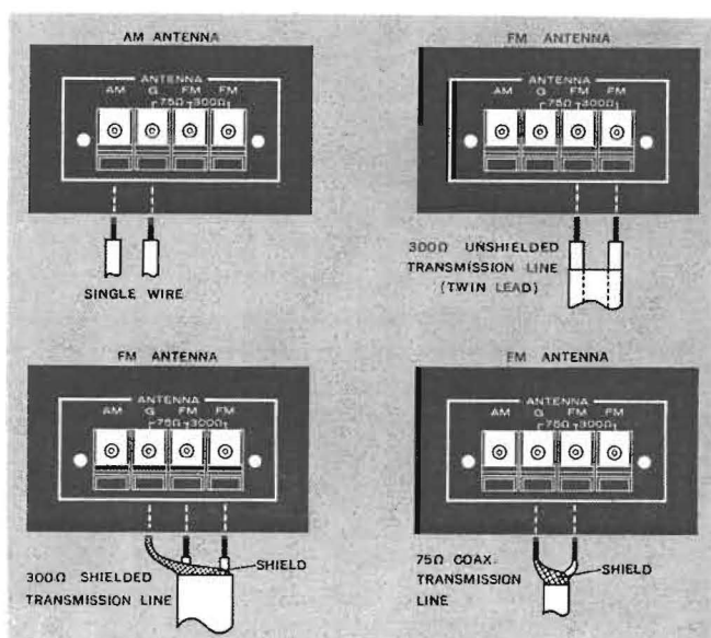
Figure 11. FM/AM Antenna Connections
