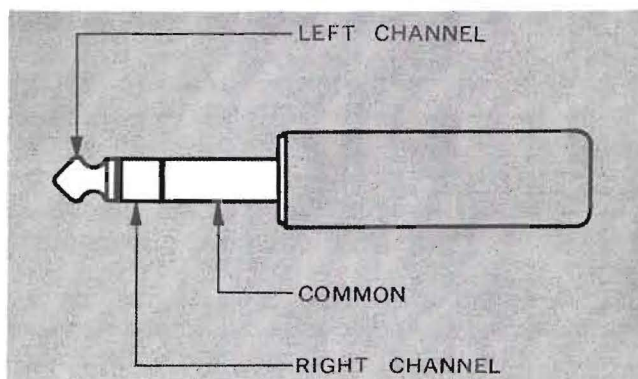
Figure 10. Stereophone Plug
