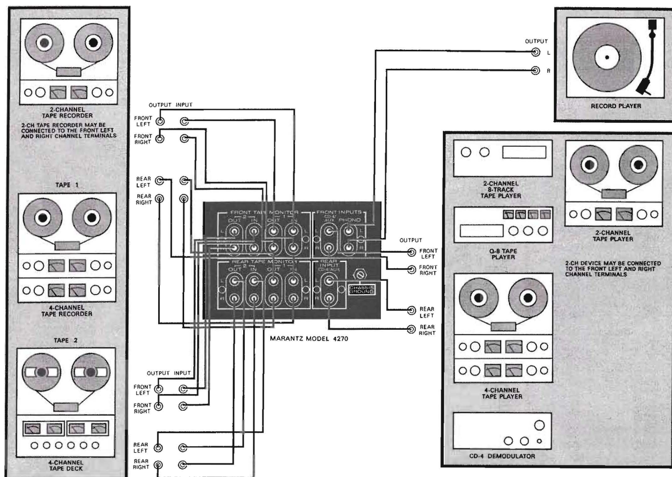
Figure 3. Connection Diagram
