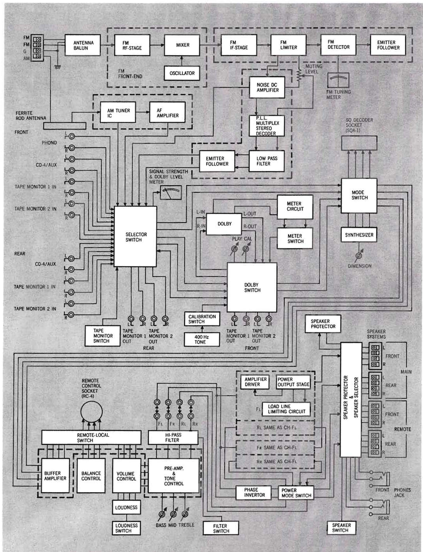
Figure 14. Block Diagram
