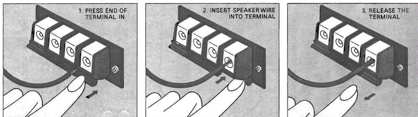
Figure 13. Quick-Connect Speaker Terminal
