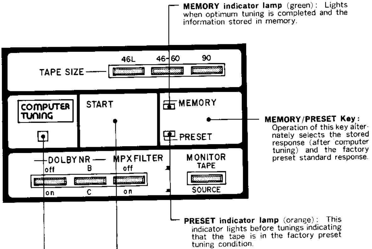
Fig. 10 START key: This begins the tuning sequence. TUNING indicator: This light flashes during the tuning sequence.
