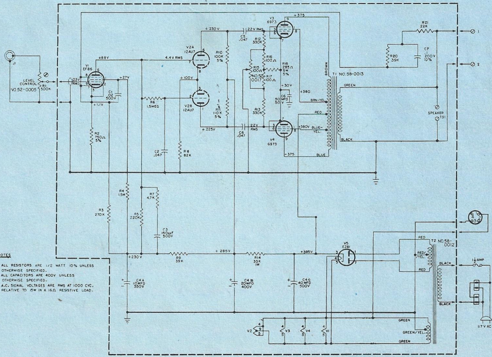
(35) 15-WATT AMPLIFIER
