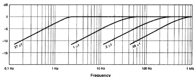
Fig. 3.4 Effect of Input Capacitor Value on Frequency Response
