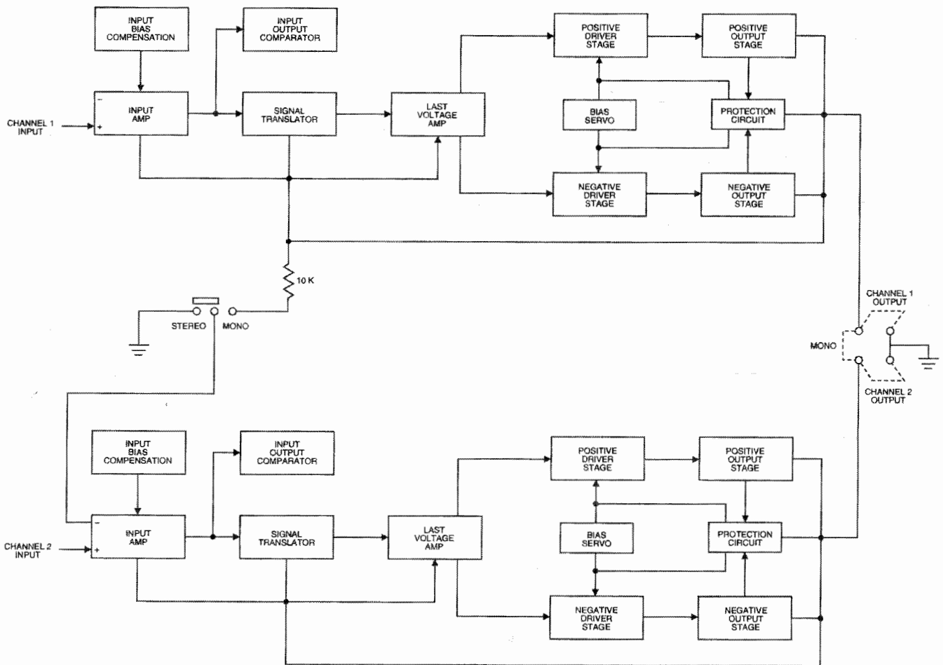
Fig. 6.1 Circuit Block Diagram
