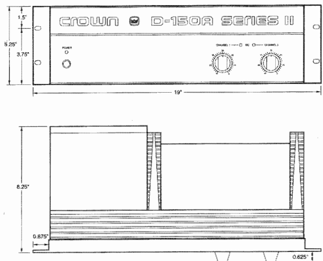
Fig. 3.2 Mounting Dimensions
