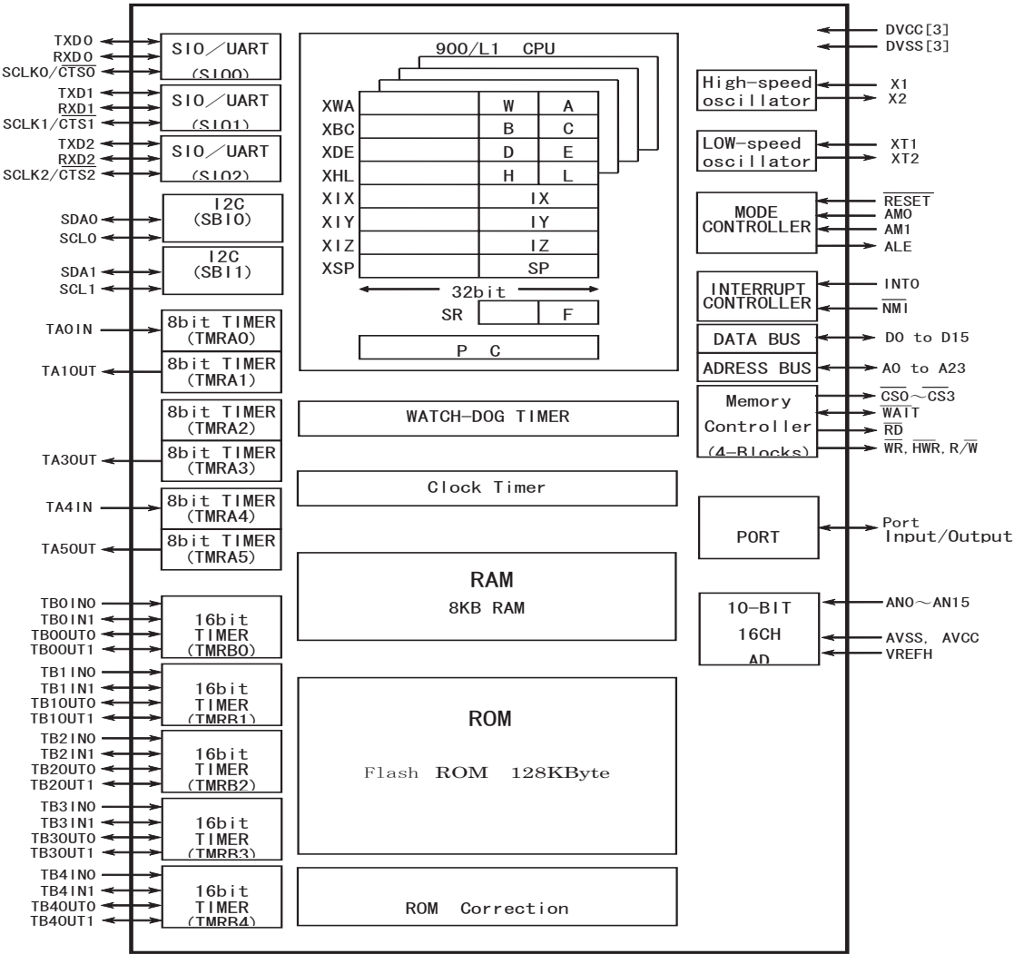
Figure 1-2 Block Diagram
