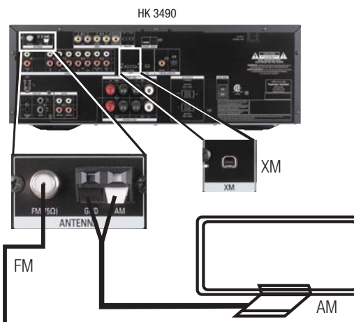
Figure 13 – Antenna Connections
