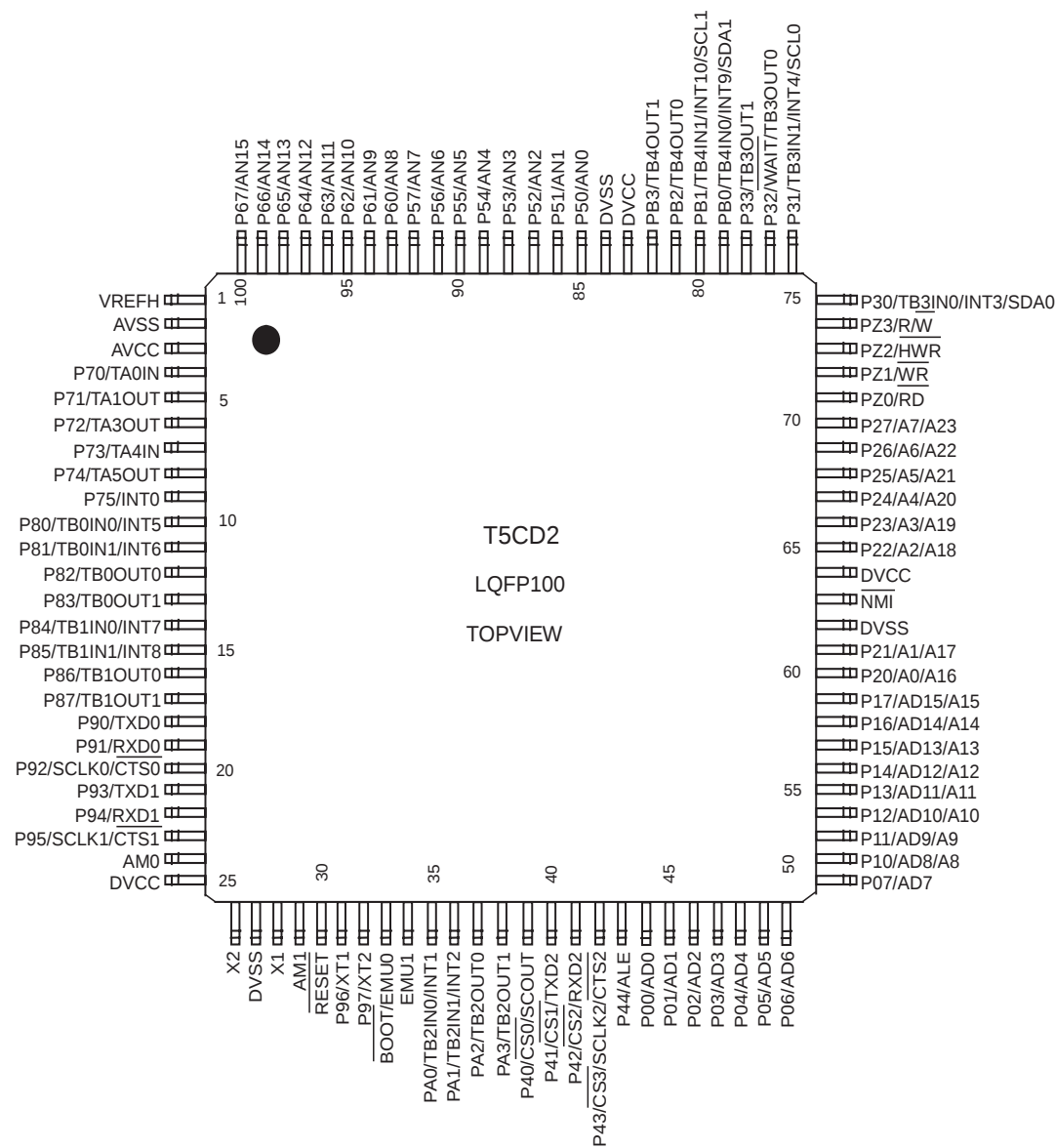
Figure 1-1 Pin Assignment
