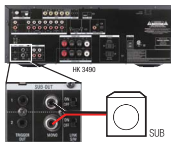
Figure 12 – Subwoofer Connection
