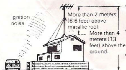
FM Outdoor Antenna Installation
