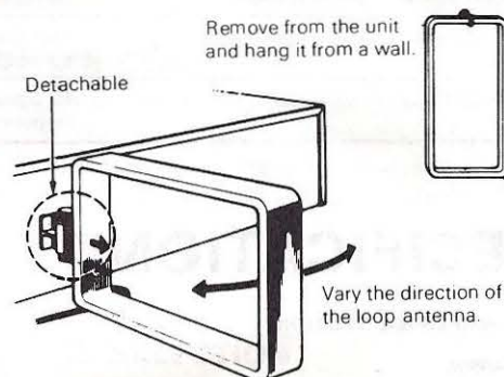
AM Loop Antenna Setting
