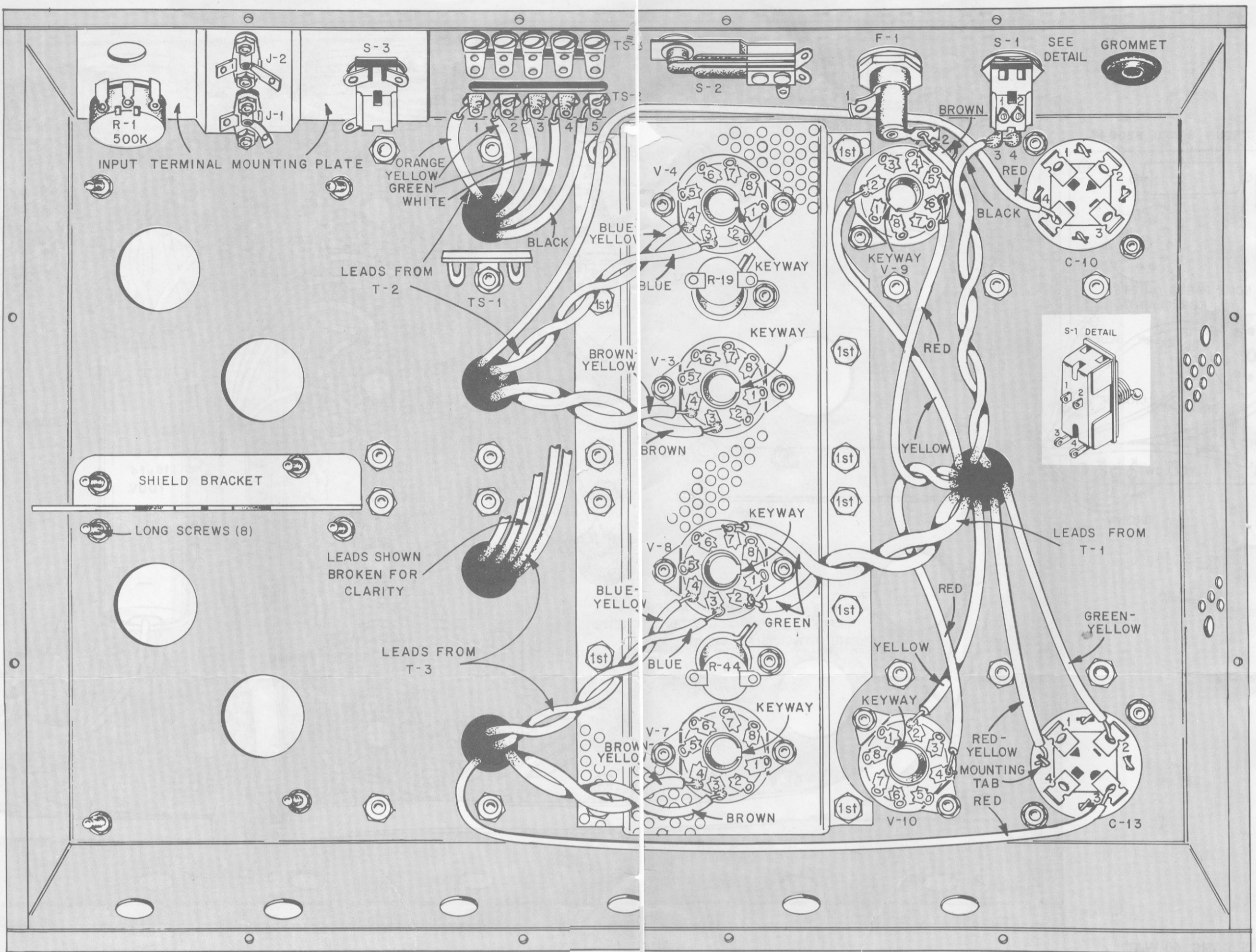
FIGURE 7. FIRST PARTS MOUNTING AND WIRING VIEW
