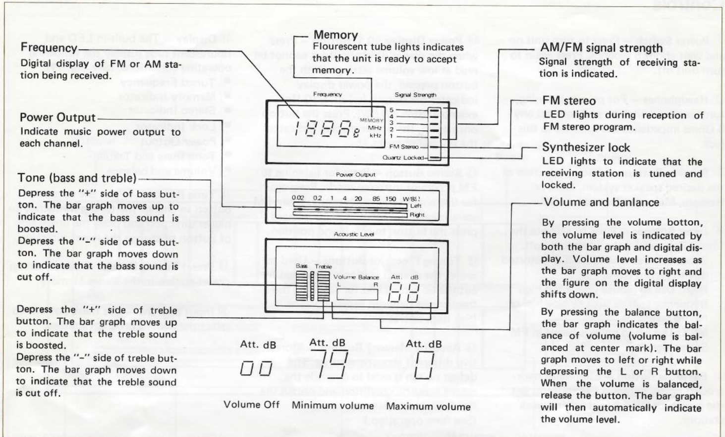
Fig. 11 Details of display unit
