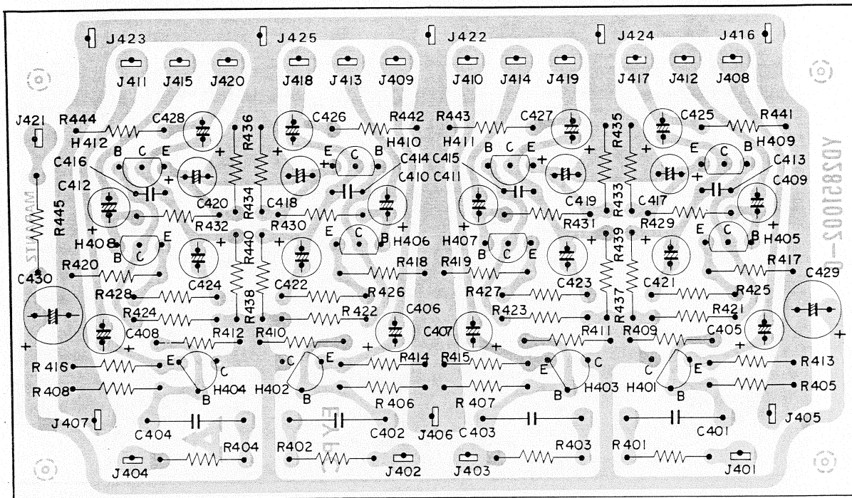
Figure 8. Tone Amplifier Assembly P400 Component Locations
