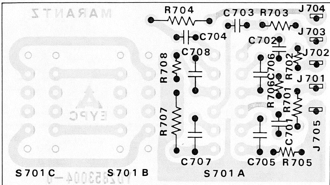
Figure 11. Loudness and Speaker Switch Assembly P700 Component Locations
