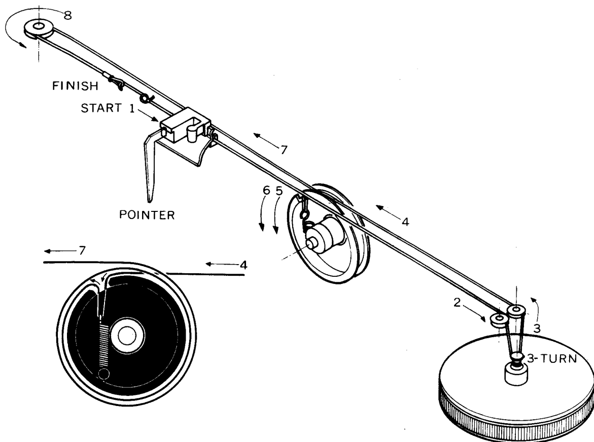
Figure 1. Dial Stringing
