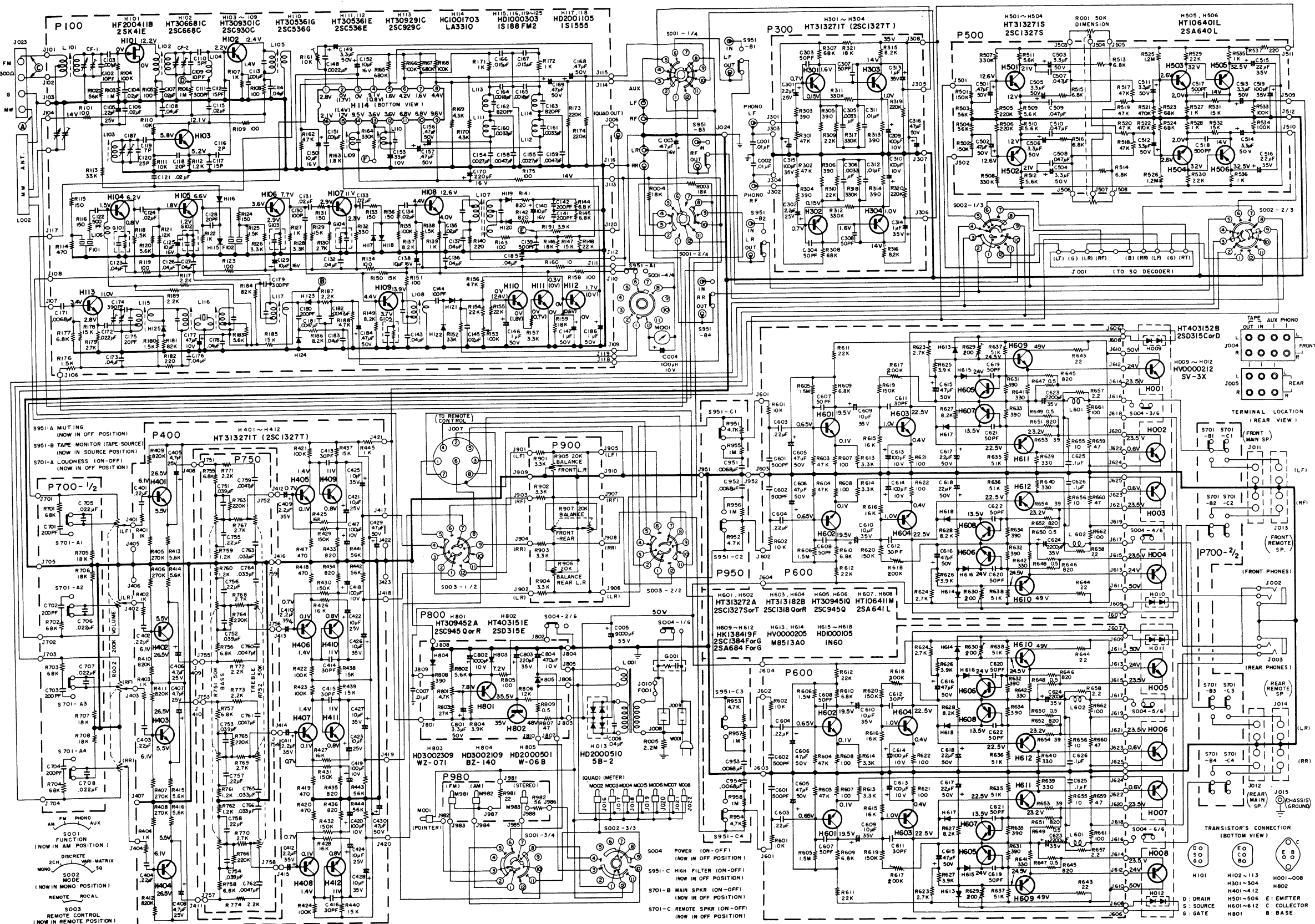
Figure 16. Schematic Diagram
