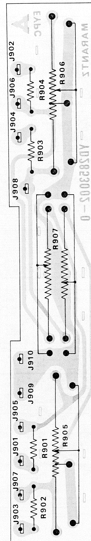
Figure 14. Balance Control Unit Assembly P900 Component Locations
