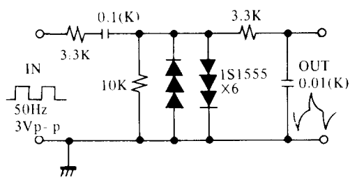
Differentiation Circuit
