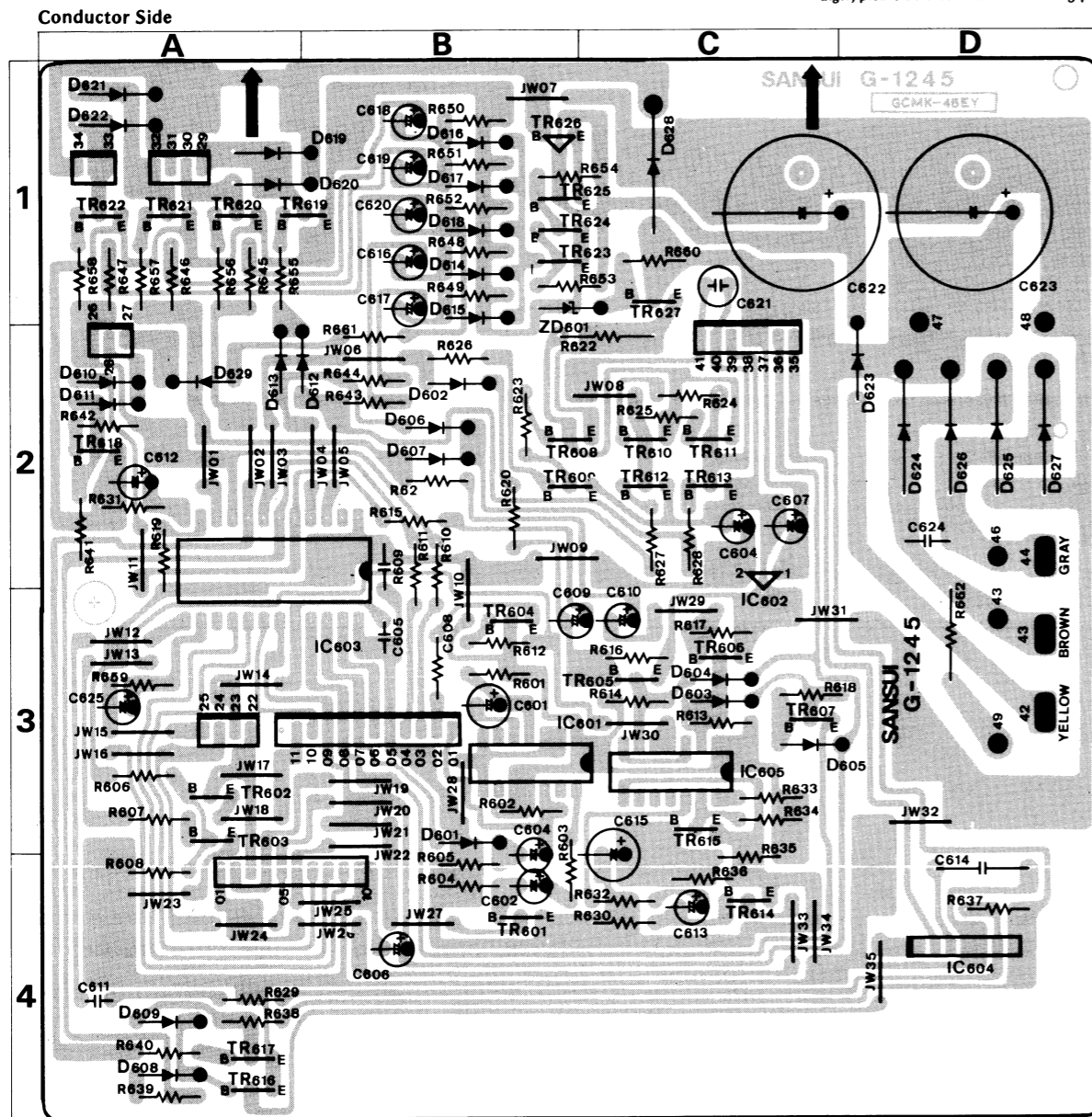
8-1. G-1245 Control Circuit Board (Stock No. 76301401)
