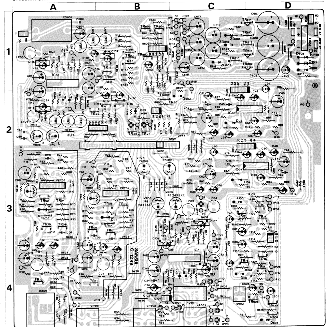
8-2. G-1249 Play & Rec Amp. Circuit Board (Stock No. 76201901)
