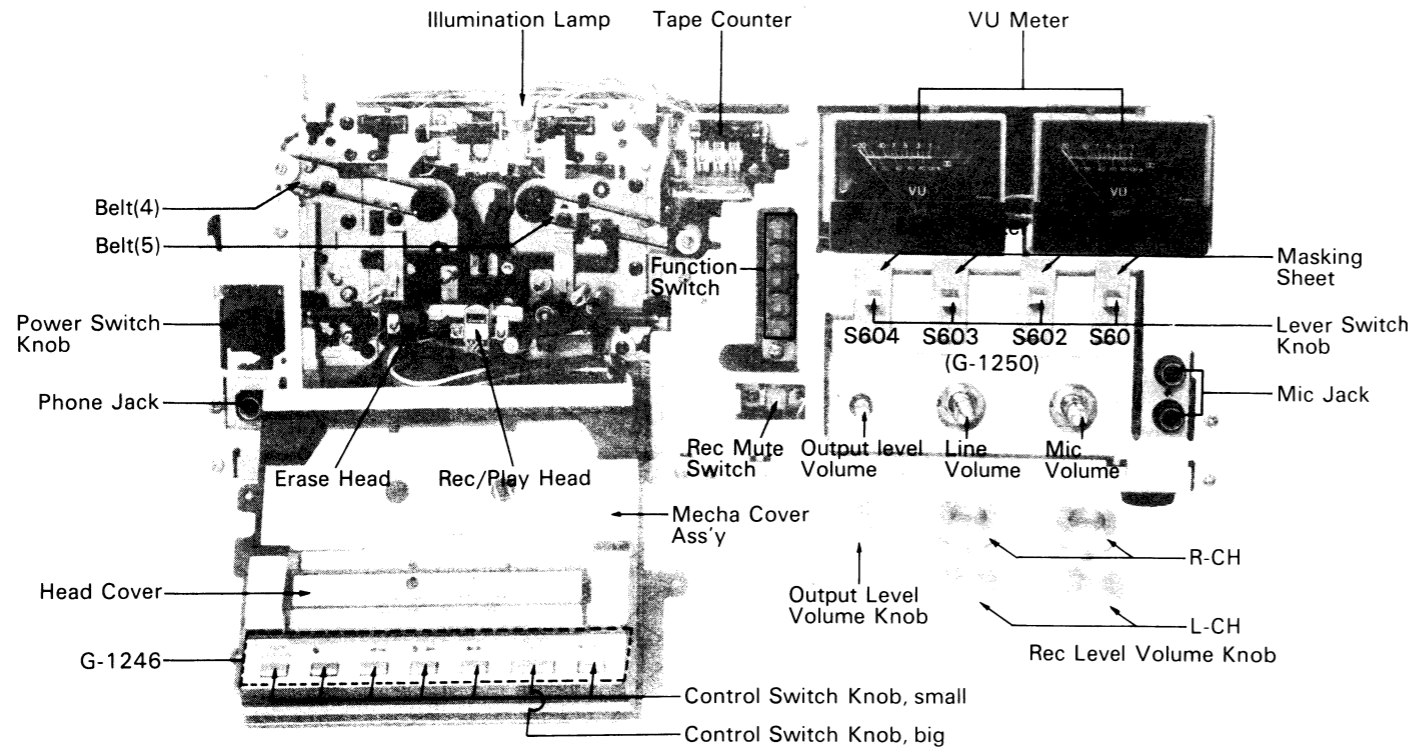
6-1. Front View
