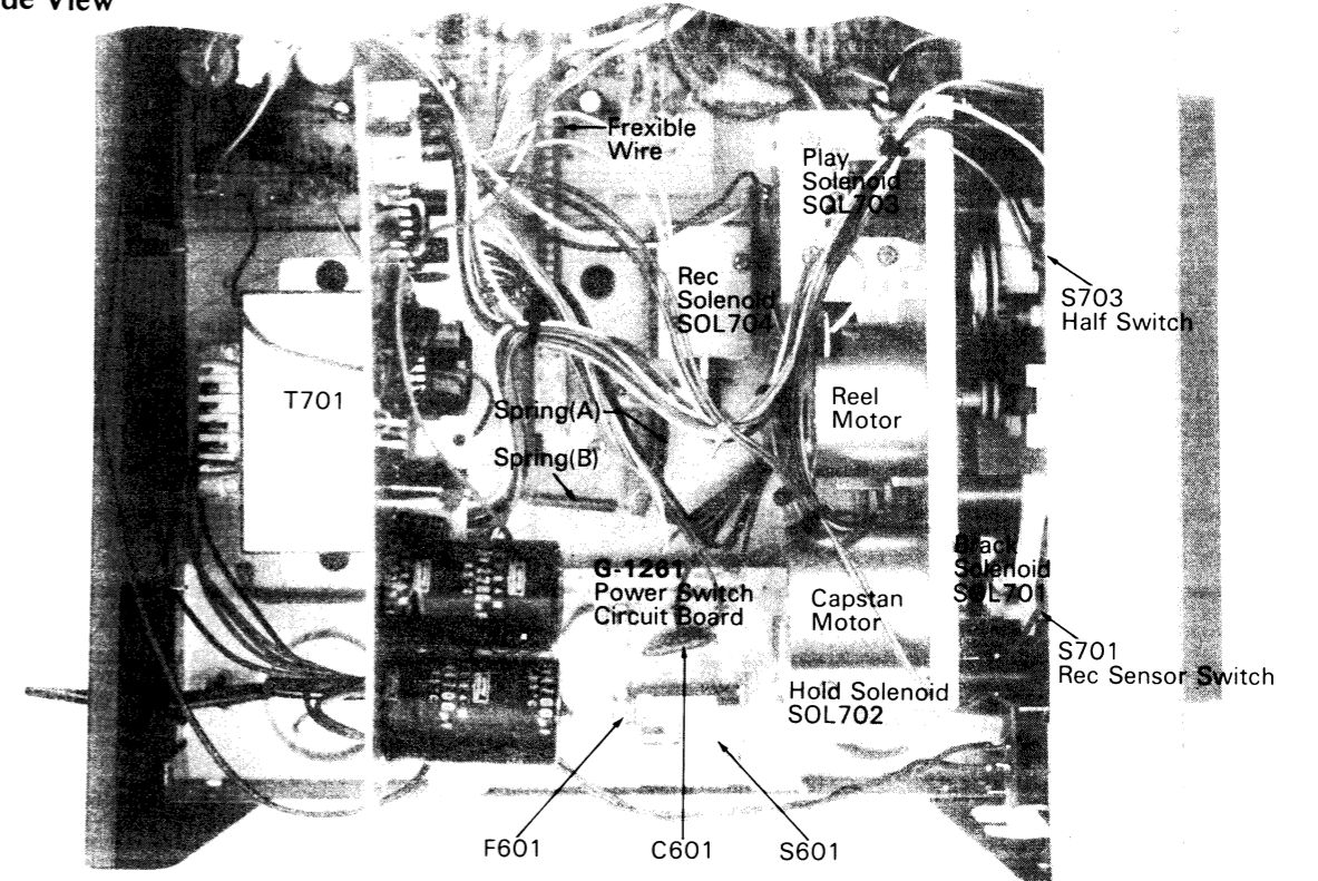
6-3. Side View
