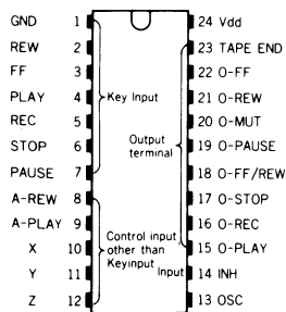
Fig. 2-1 Top view & pin function of IC TC-9121P
