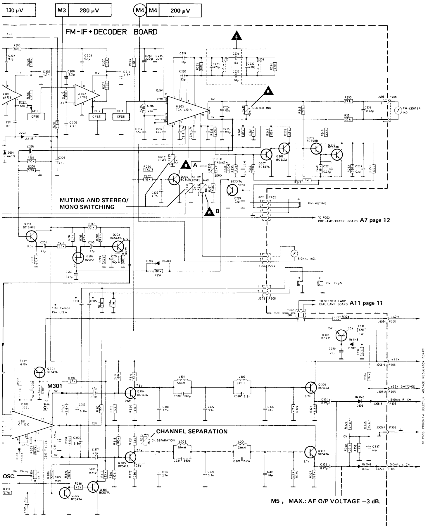
FM-IF SECTION - 43617
