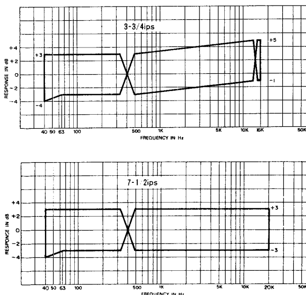
Fig. 8-10 Frequency Response - OVERALL - 1
