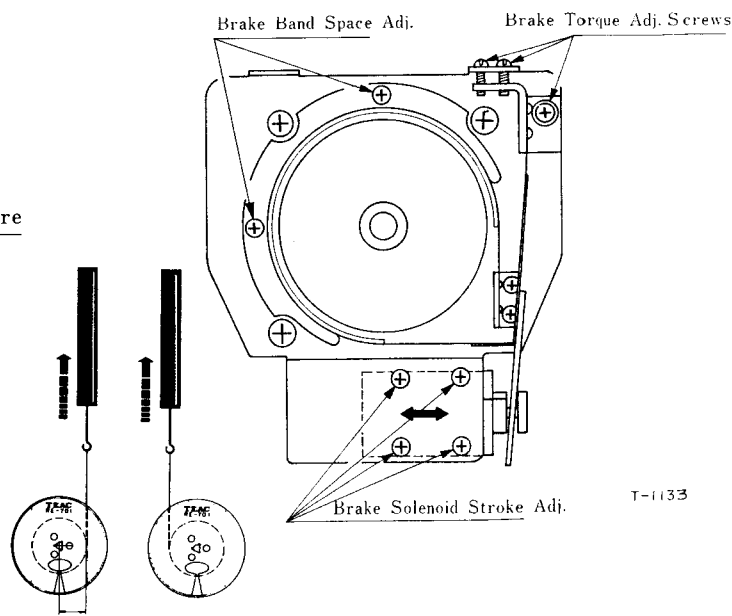
Fig. 7-2 Torque Measurement and Adjustment Location
