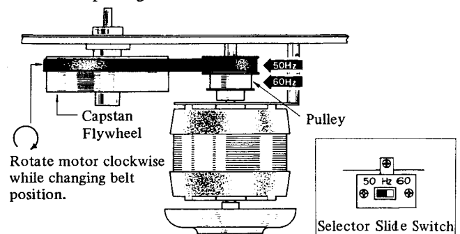
Fig. 7-6 Frequency Conversion
