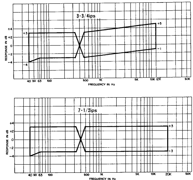
Fig. 8-11 Frequency Response - OVERALL - 2
