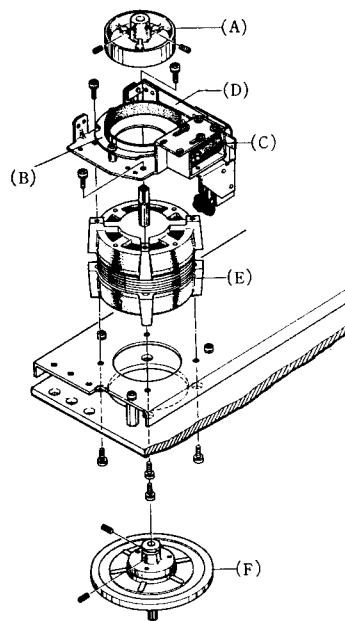
Fig. 4-5 Reel Motors Removal
